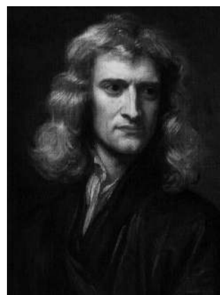
Figura 1: Isaac Newton
